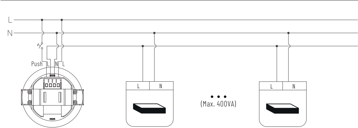
CONNECTION DIAGRAM
