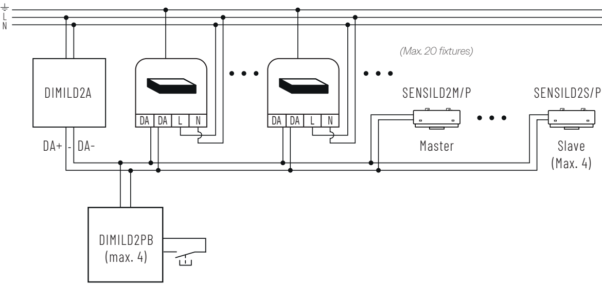
CONNECTION DIAGRAM
