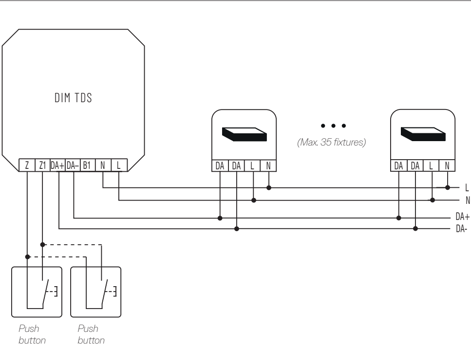
CONNECTION DIAGRAM
